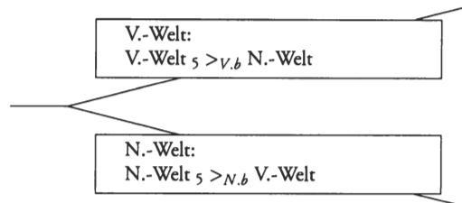
Abb. 2: Vermeer-Novalis-Situation T
