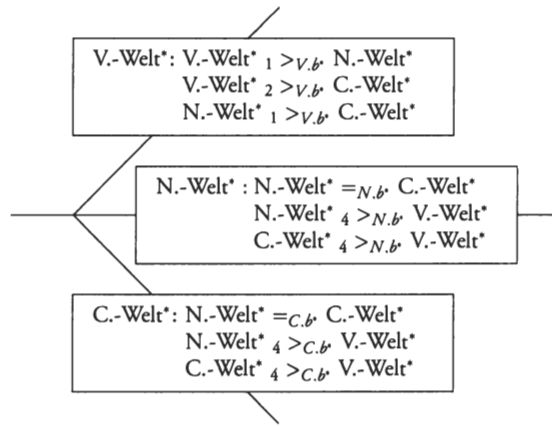
Abb. 3: Vermeer-Novalis-Chopin-Situation T*
